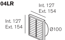
Flat Duct Low Resistance Fixed Louvre PP2-104LR
